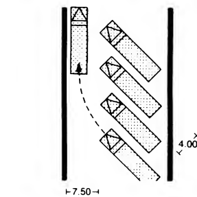
⑤ Parking at less than 45°
